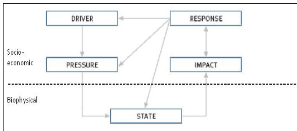
Figure 23.1 THE DPSIR FRAMEWORK
