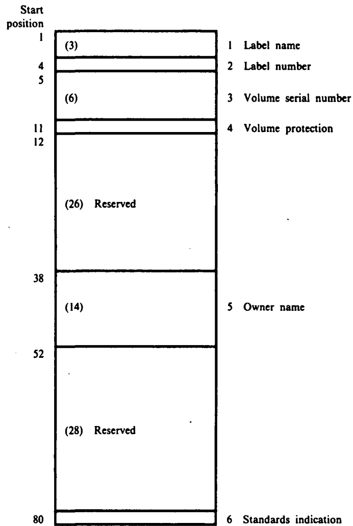
Figure A.5 ANSI volume label
